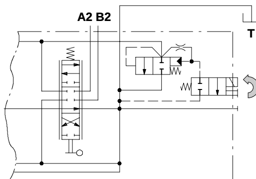
Normally closed configuration type ELC
