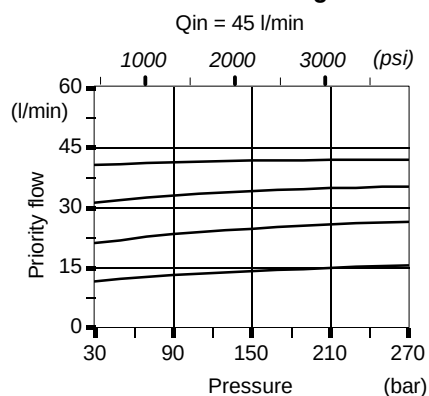
Pressure-flow diagram
