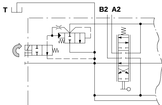
Normally open configuration type EL
