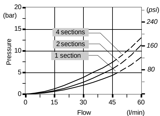
Pressure drop A(B)→T on 4 sections directional valve
