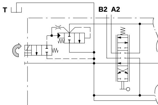
Normally closed configuration type ELC
