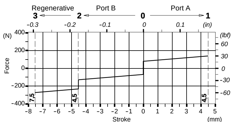
Force-stroke diagram
