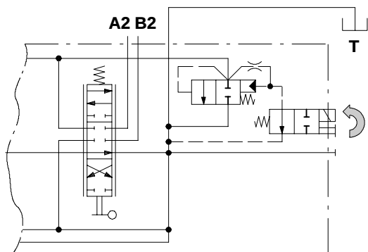
Normally open configuration type EL
