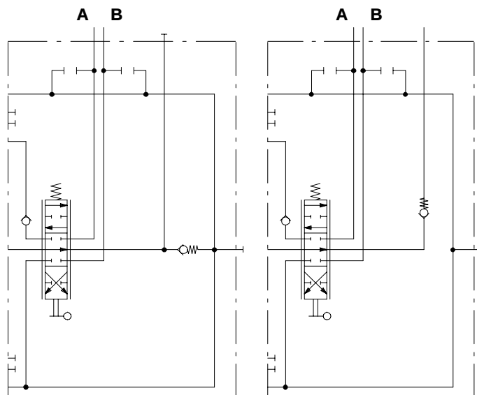
Type RPA: with port valves prearrangement
