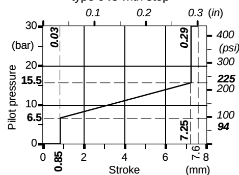
Pressure control curve (port VB2) type 045 with step
