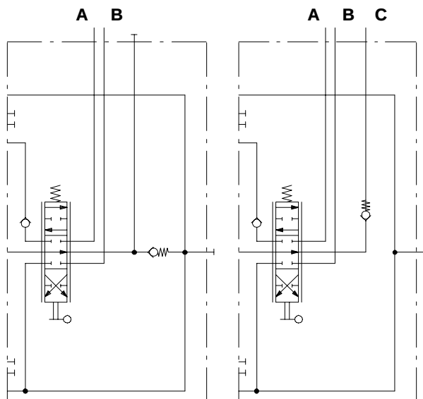
Type RQA: without port valves prearrangement
