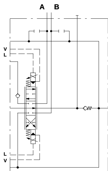
Description example: RPE-E101-8EB3.UTUT-VRC-F-12VDC
