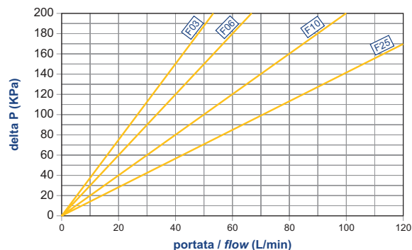
BY-PASS / BY-PASS
